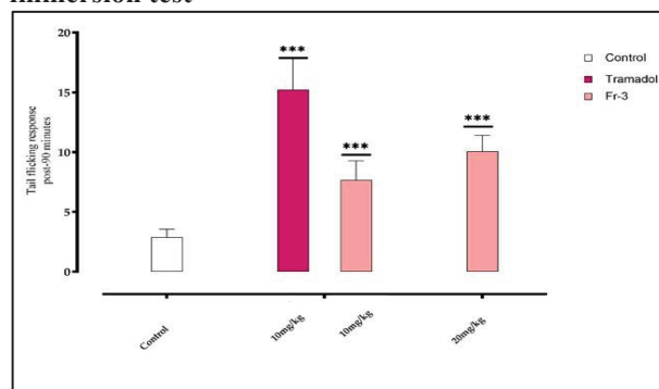
Figure 5: The analgesic effect of chalcone using tail immersion test
