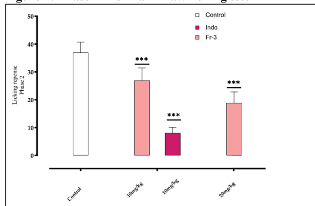
Figure 4: Phase 2- Formalin Paw licking test
